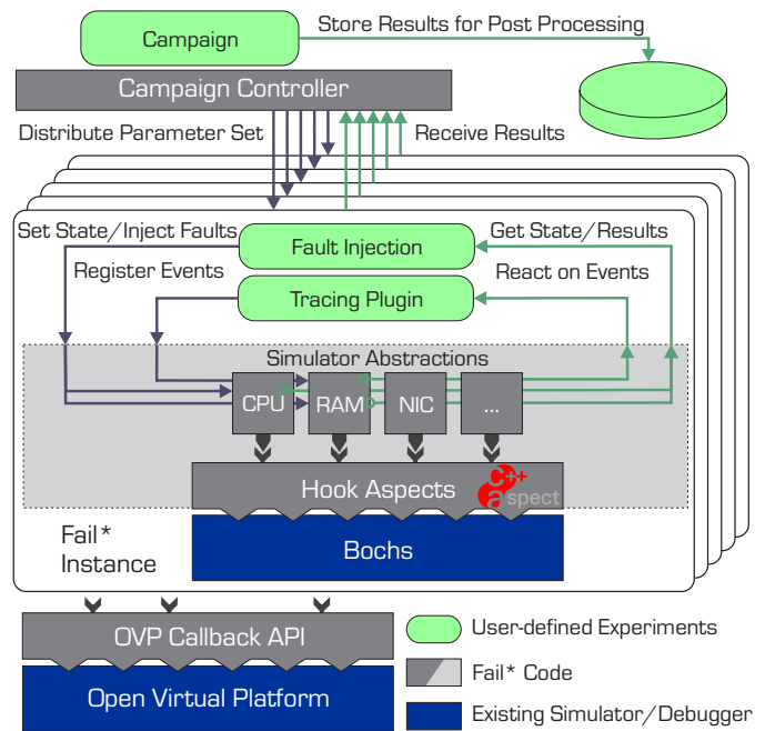
Figure 1. Architecture overview: The Campaign Controller distributes parameter sets from a user-defined Campaign throughout the FAIL* instances. Each single experiment (“ Fault Injection ”) consumes a parameter set, and controls its target backend through a Simulator Abstraction layer. Actual target backends (simulators, but also real prototype hardware) can be exchanged by providing an interfacing module to this abstraction.
